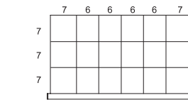
R_GE-A0512_ _ 18 COMPARTIMENTS
