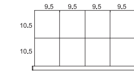
R_GE-A0304_ _ 8 COMPARTIMENTS
