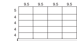
R_GE-A0316_ _ 20 COMPARTIMENTS
