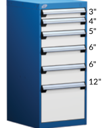
6 TIROIRS L3ABD-4029__ 18" x 21" x 40" L3ABG-4029__ 18" x 27" x 40"
