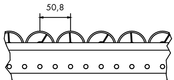
Wheel pitch
