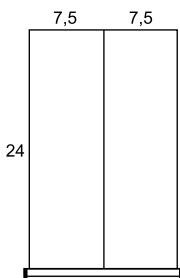
L__BG-A0100__ 2 compartiments
