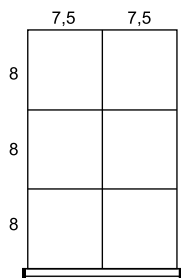
L__BG-A0104__ 6 compartiments
