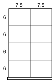
L__BG-A0106__ 8 compartiments
