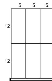
L__BG-A0203__ 6 compartiments
